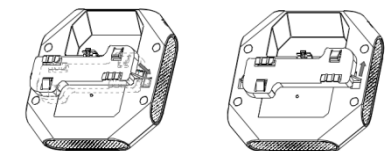
Figure 4: Attaching Ceiling Mounting Bracket
