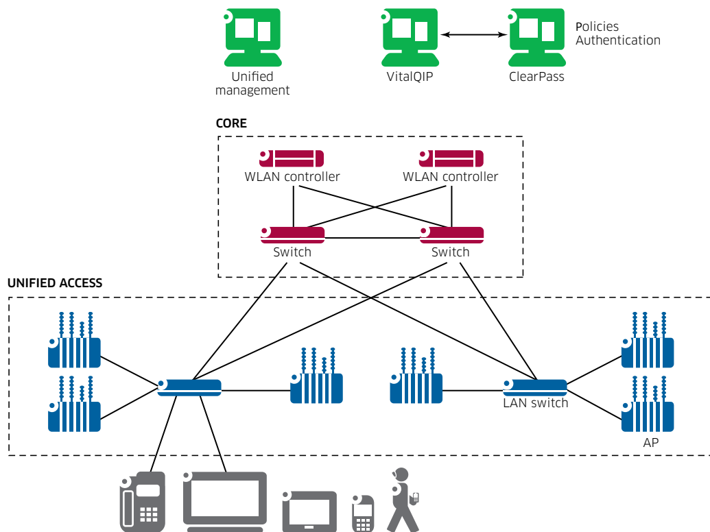
Figure 5. Unified access on the Alcatel-Lucent Enterprise Converged Campus Network Solution is governed by a policy management platform
