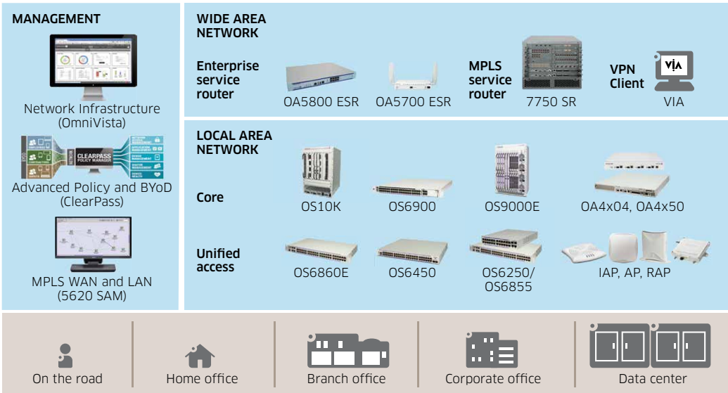
Figure 2. The Alcatel-Lucent Enterprise Converged Campus Network Solution supports BYOD with products and solutions that enable application fluency
